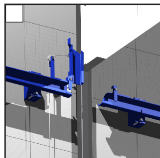
Door rail on wall, cut NOT allowed:
