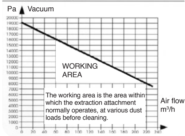
Performance curve
