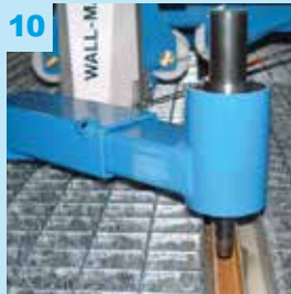
10 Floor guidance of lower support wheels.
